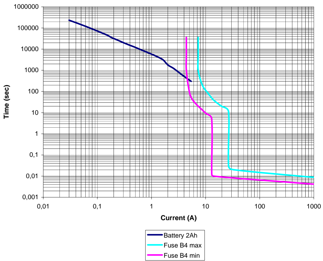
The load curve BN-24/2Ah
