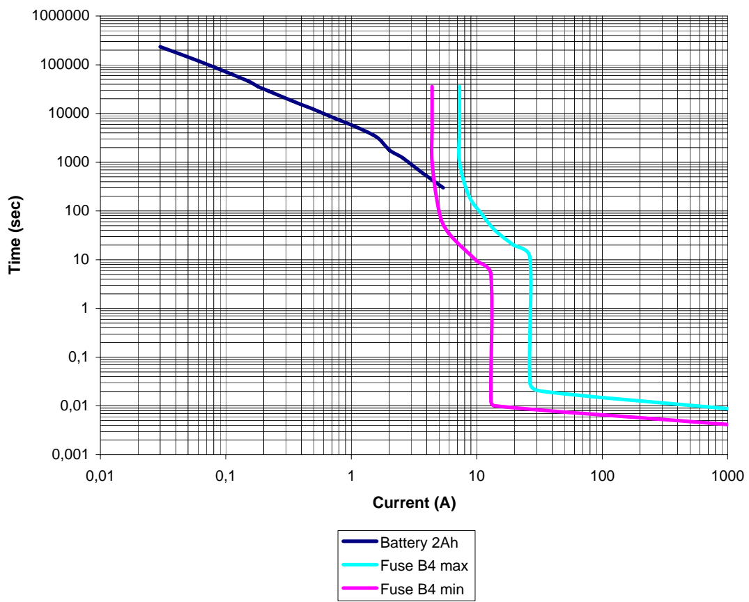
The load curve BN-48/2Ah
