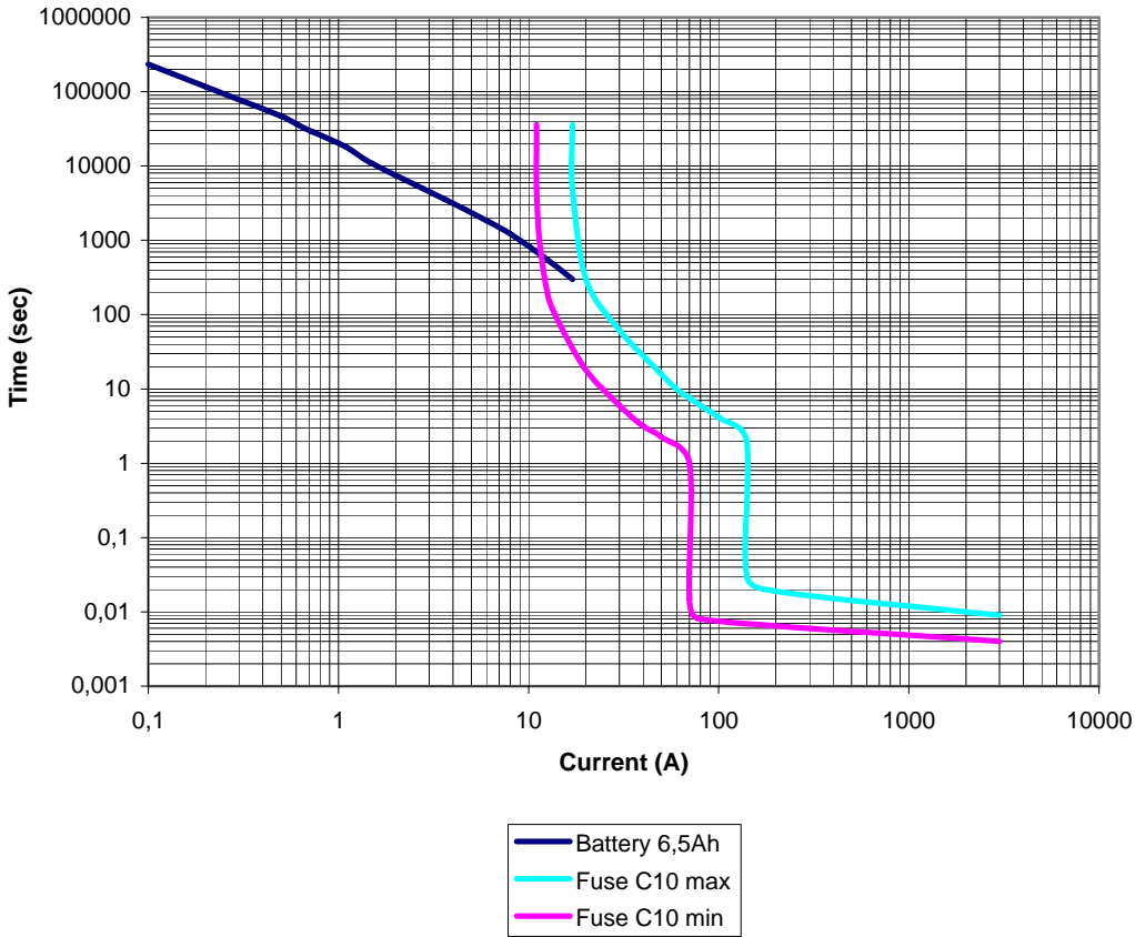
The load curve BN-48/7Ah
