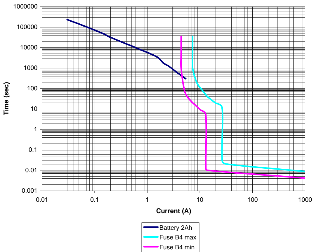
The load curve BN-110/2Ah
